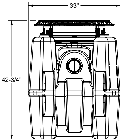
INLET END VIEW
