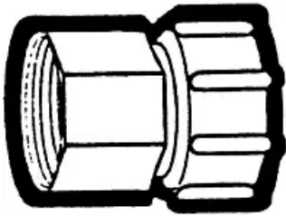
Item # 1055-12FPFH, Die Cast Nut Female Garden Hose to Female Pipe Swivel Adapter
