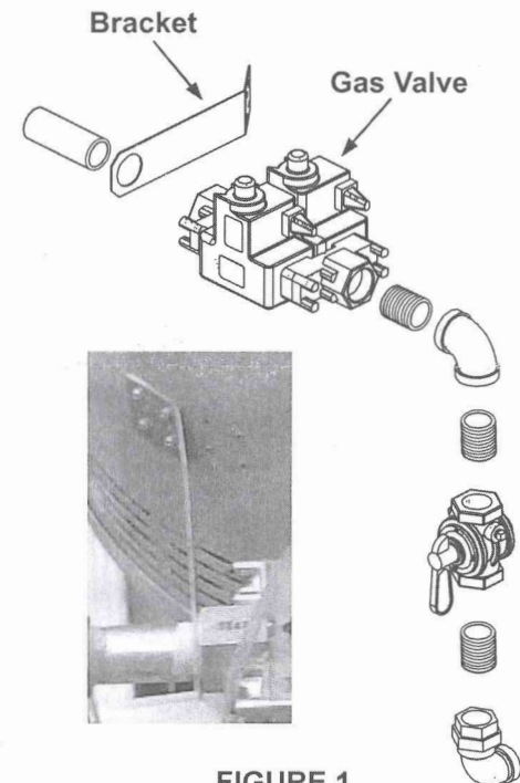
FIGURE 1. VALVE AND BRACKET ASSEMBLY
