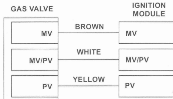
FIGURE 2. VALVE WIRING
