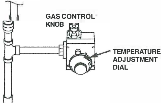
TYPICAL GAS CONTROL SHOWN.
